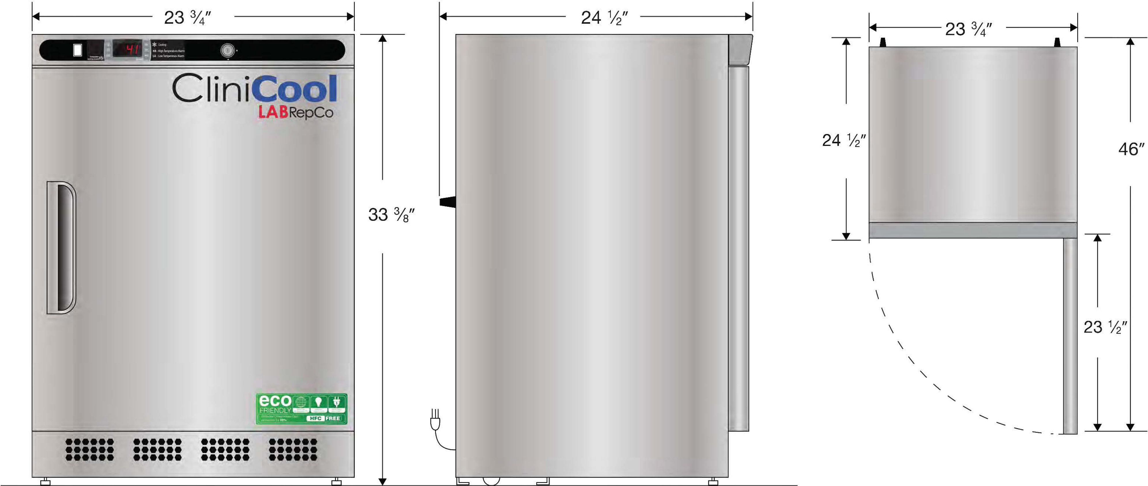
Front View
