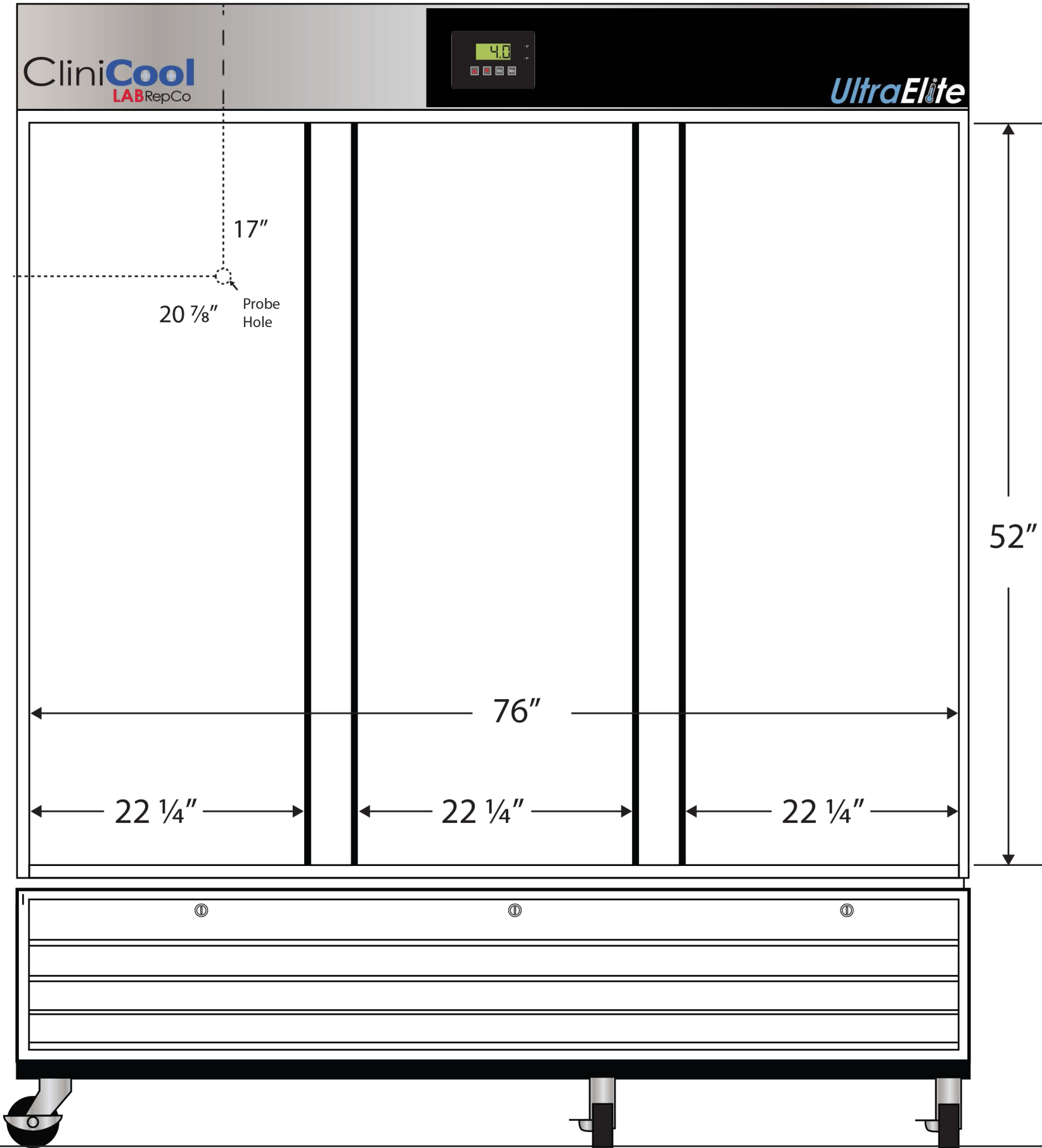
Front View
