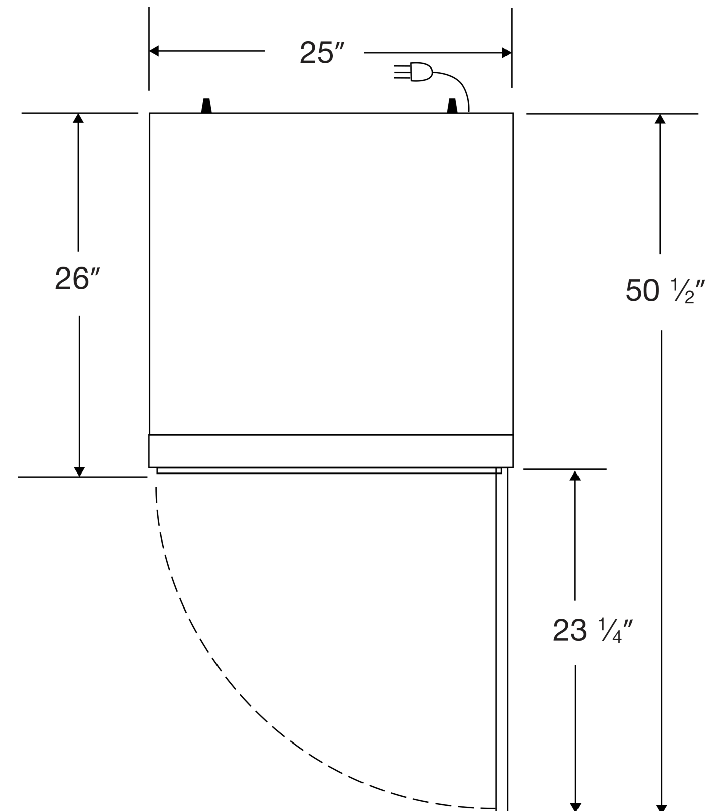
Top View
