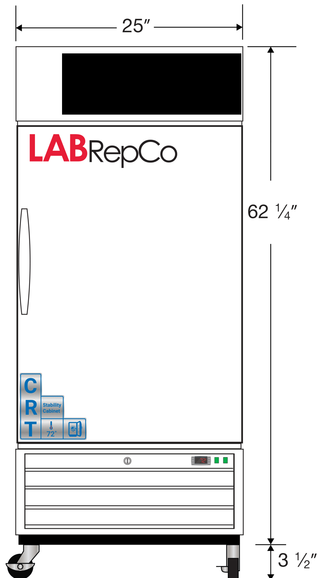
Front View
