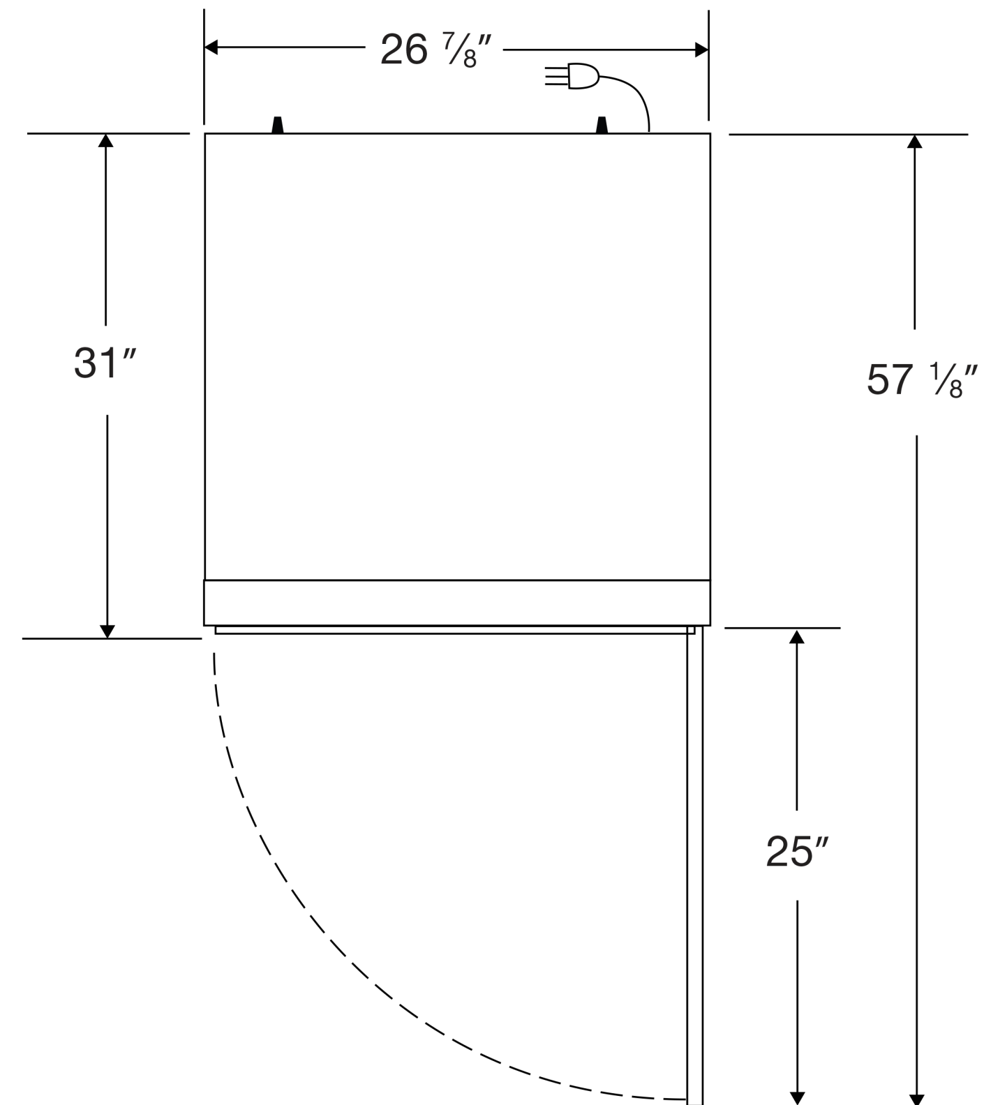
Top View
