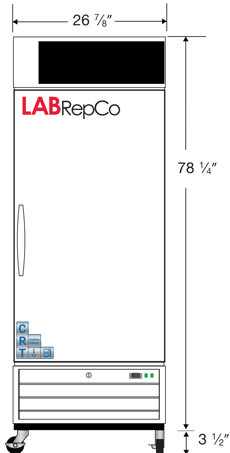
Front View
