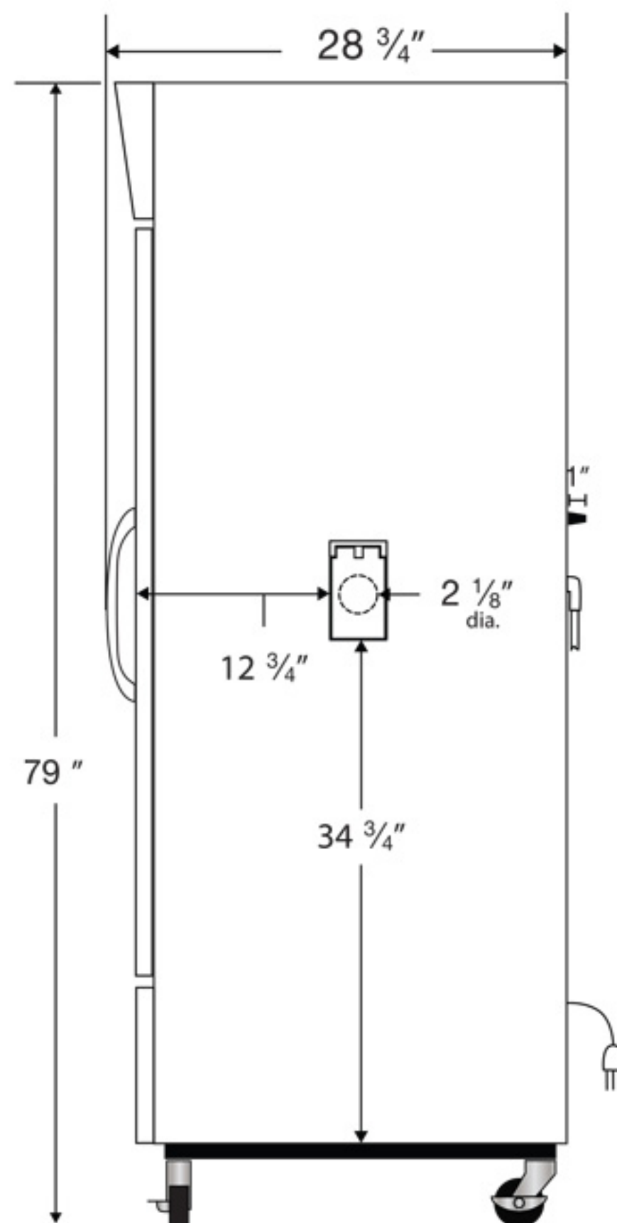
Side View
