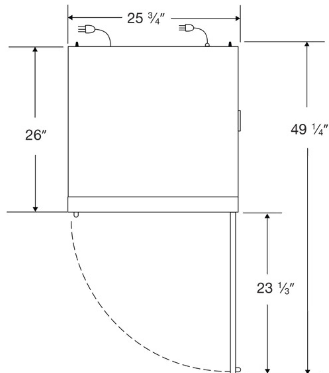
Top View
