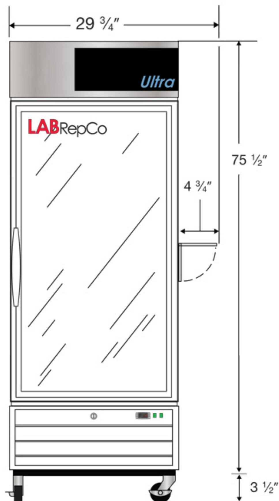
Front View
