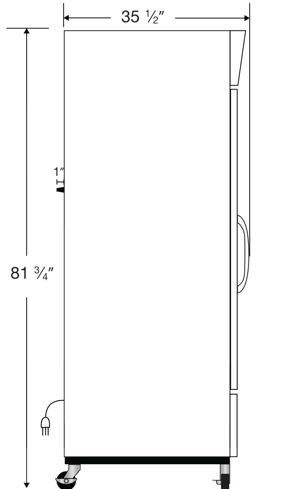
Side View
