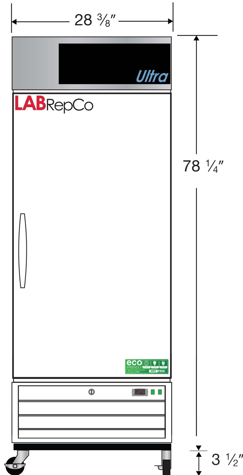
Front View
