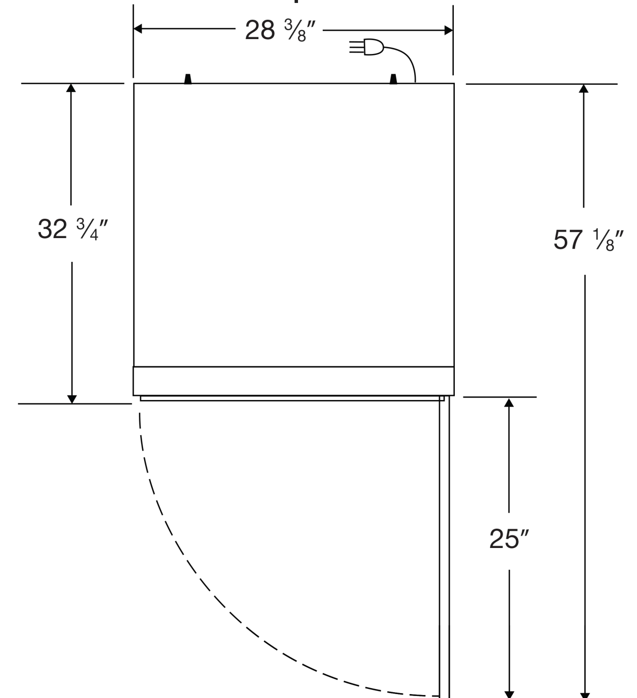
Top View
