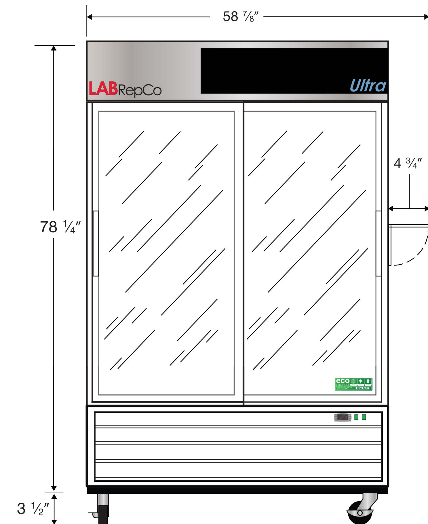
Front View
