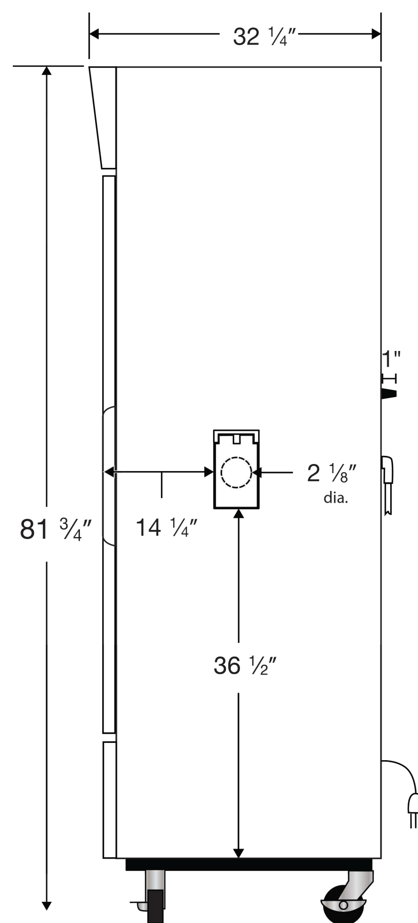
Side View
