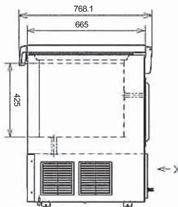
Side
