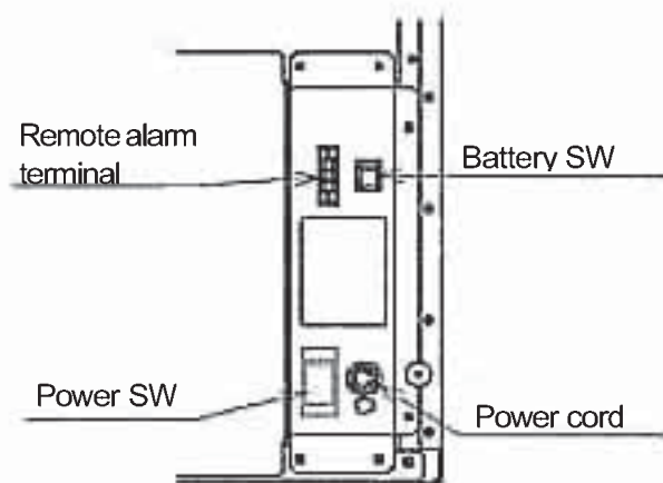
Back-right side
