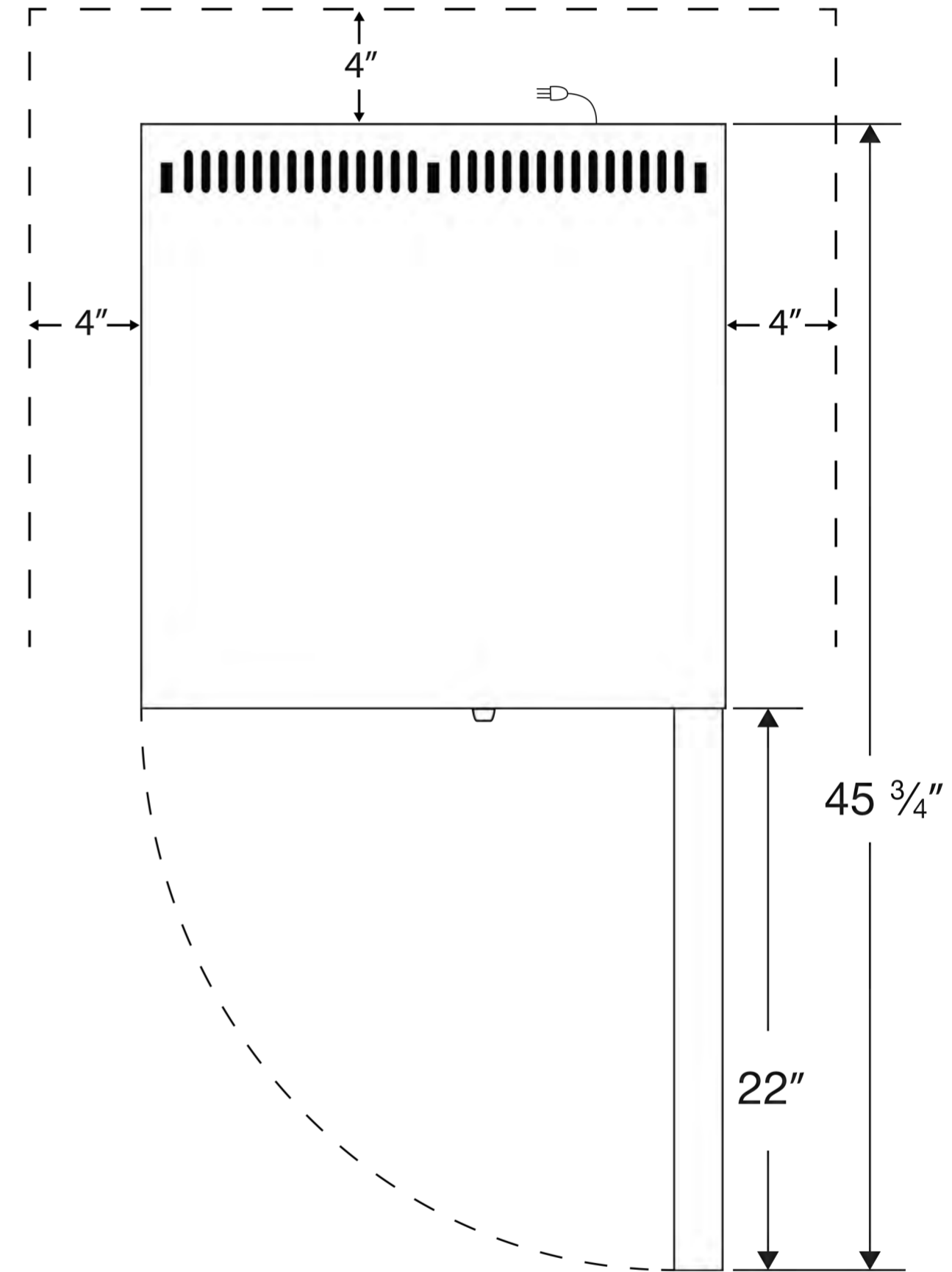
Top View
