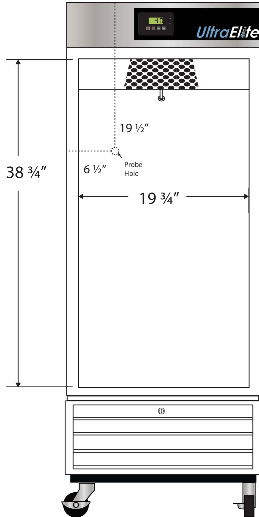
Front View
