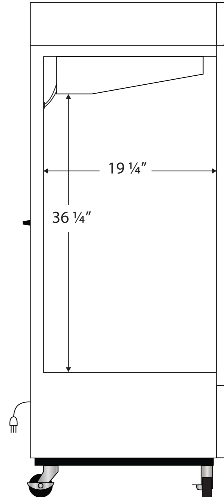
Side View
