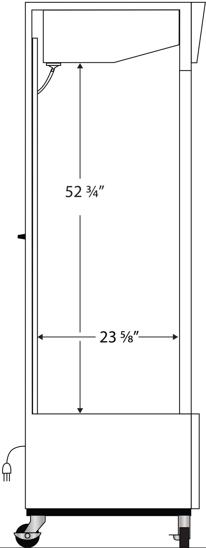
Side View
