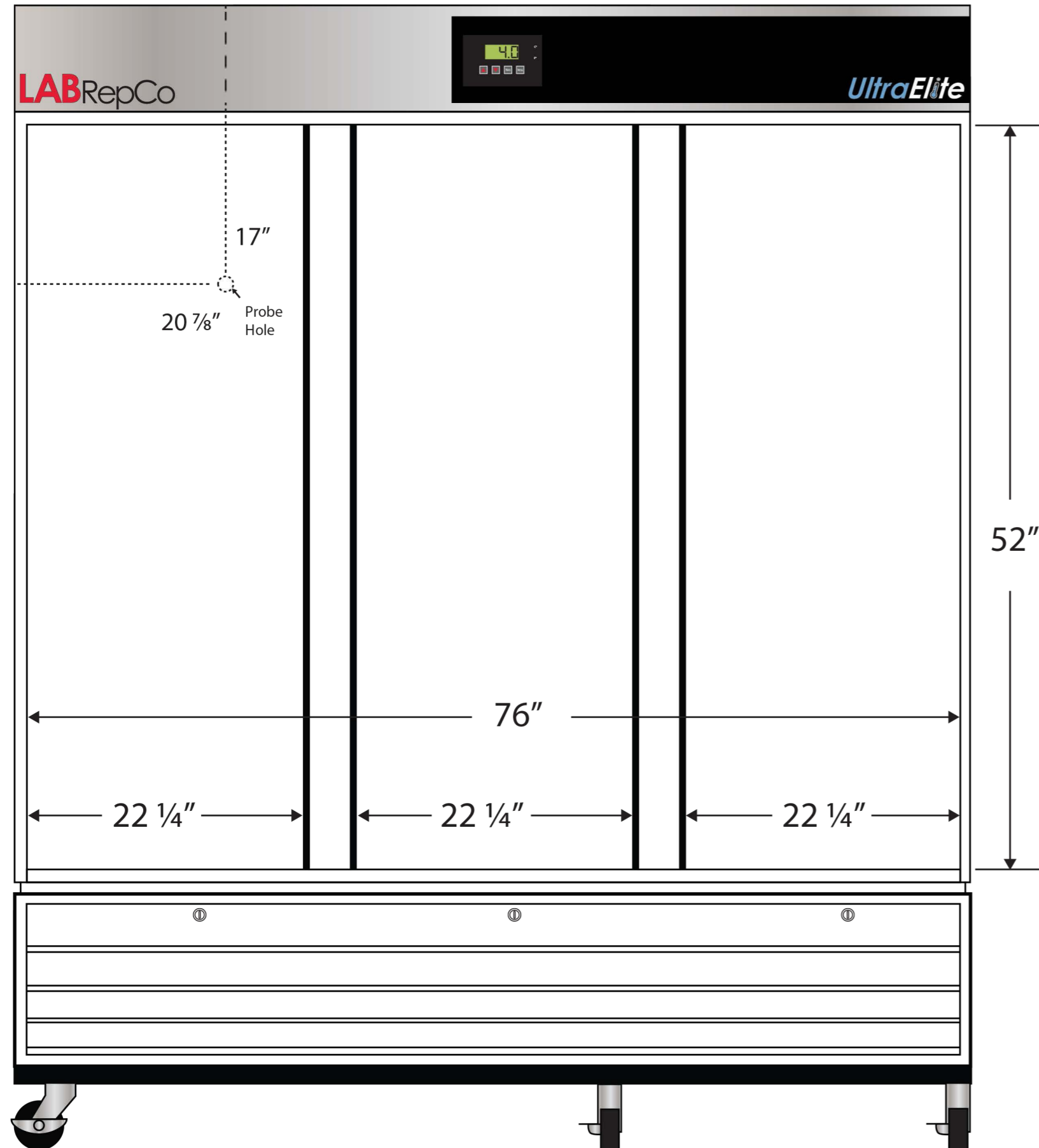
Front View
