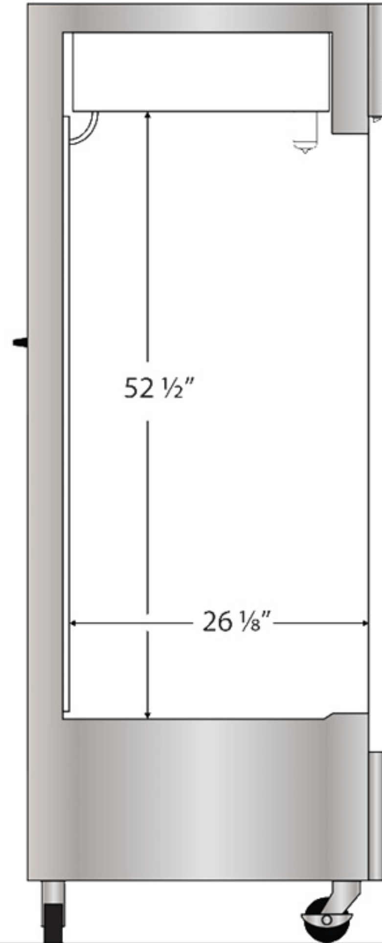
Side View
