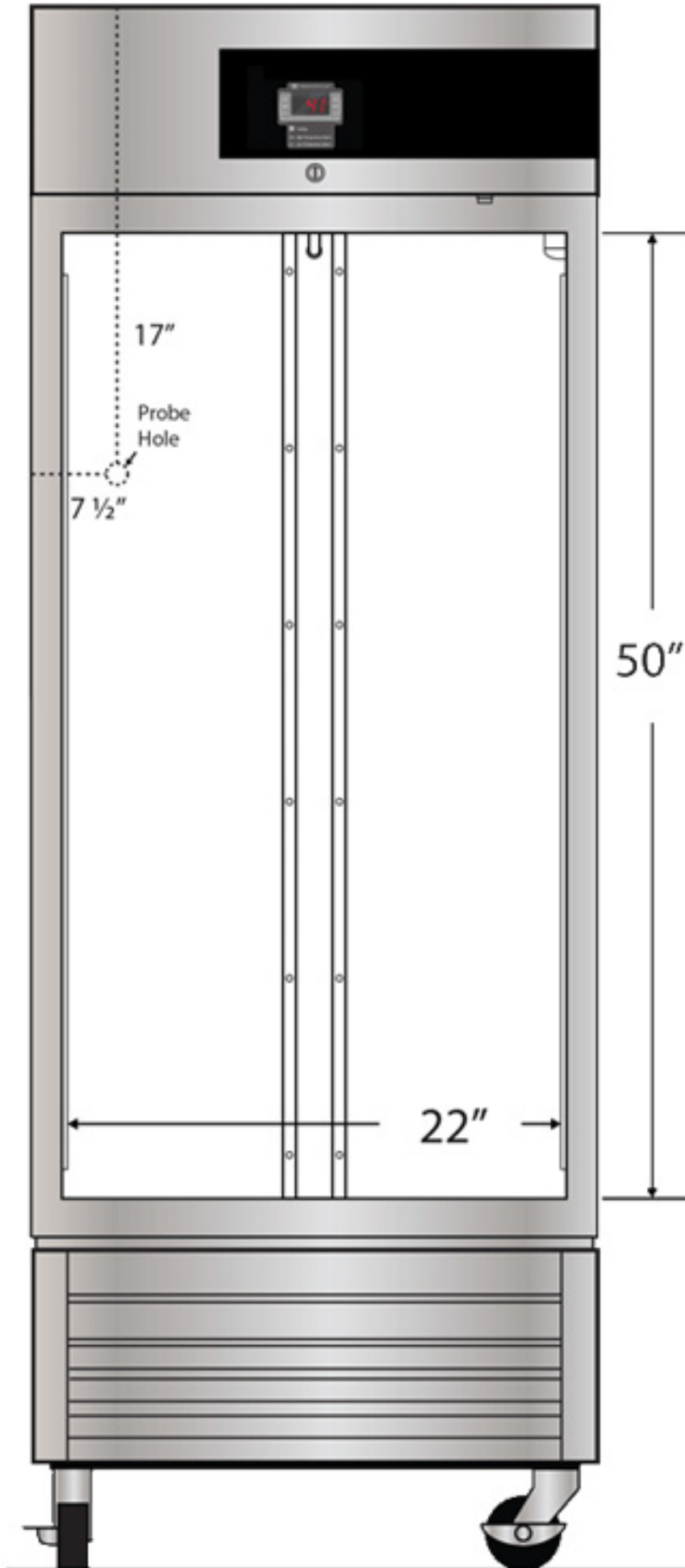
Front View
