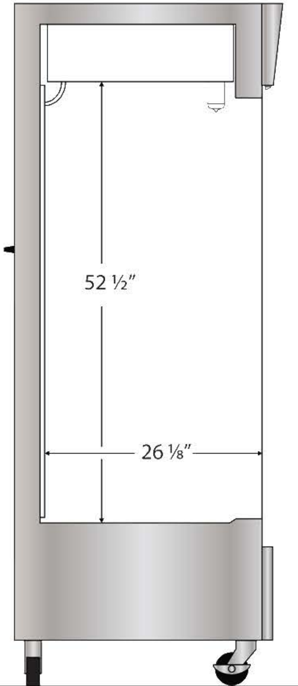
Side View
