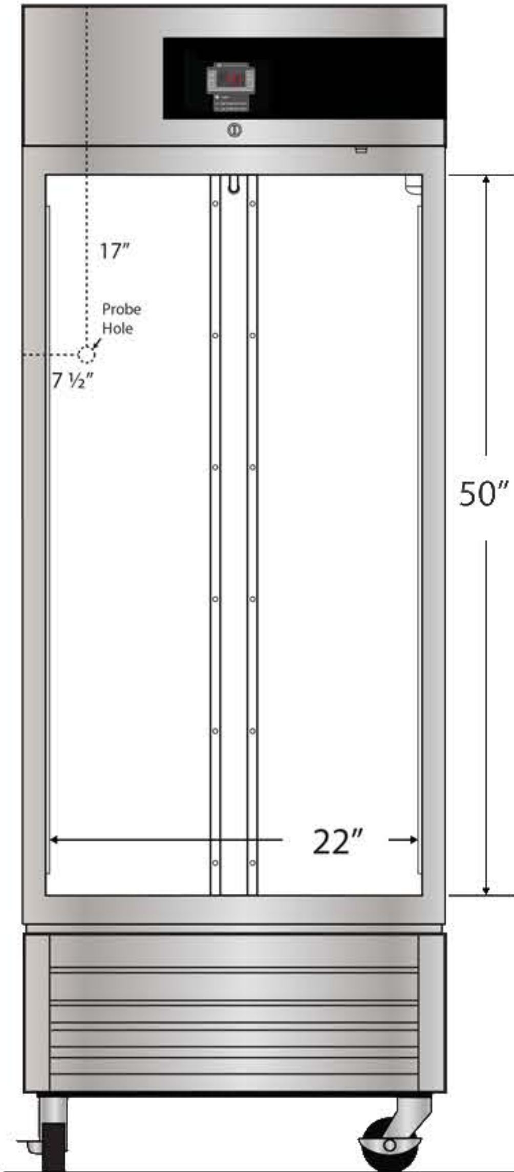
Front View
