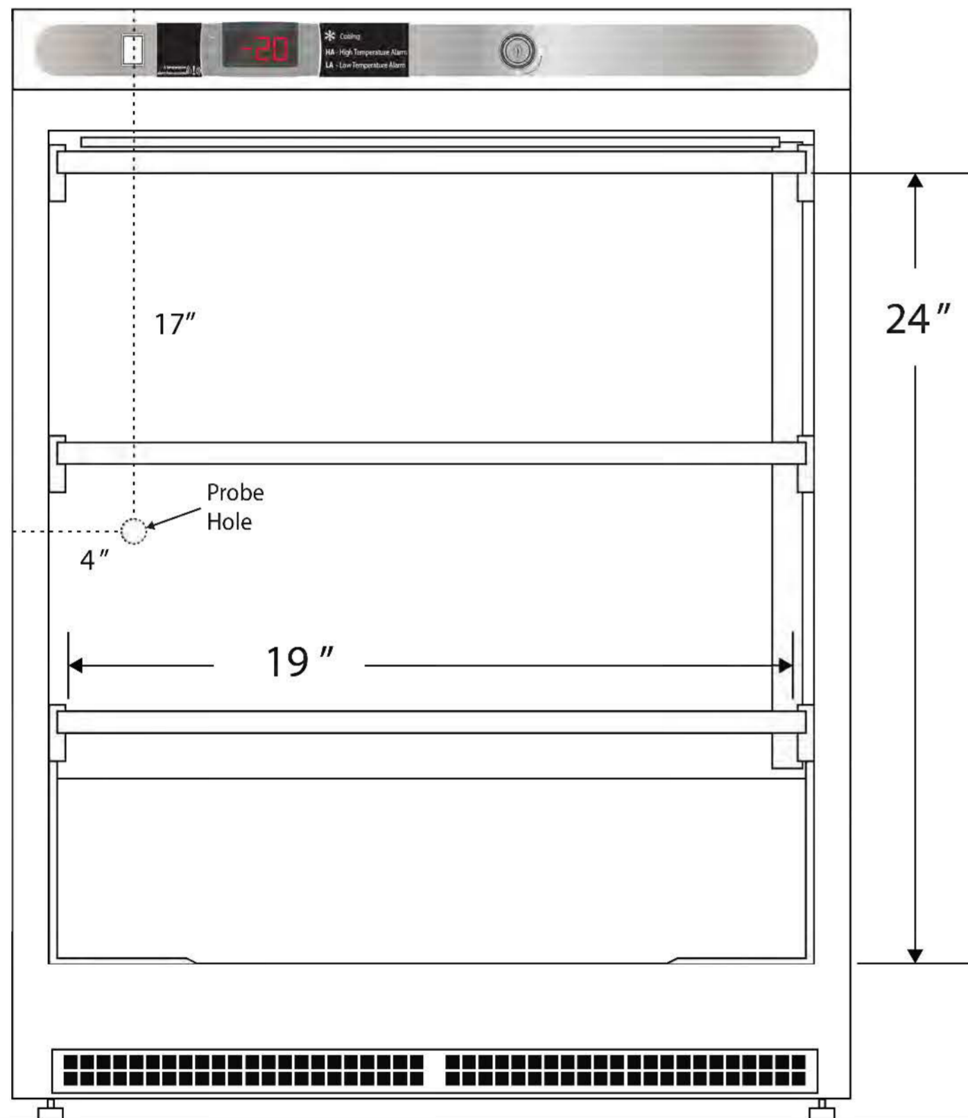
Front View
