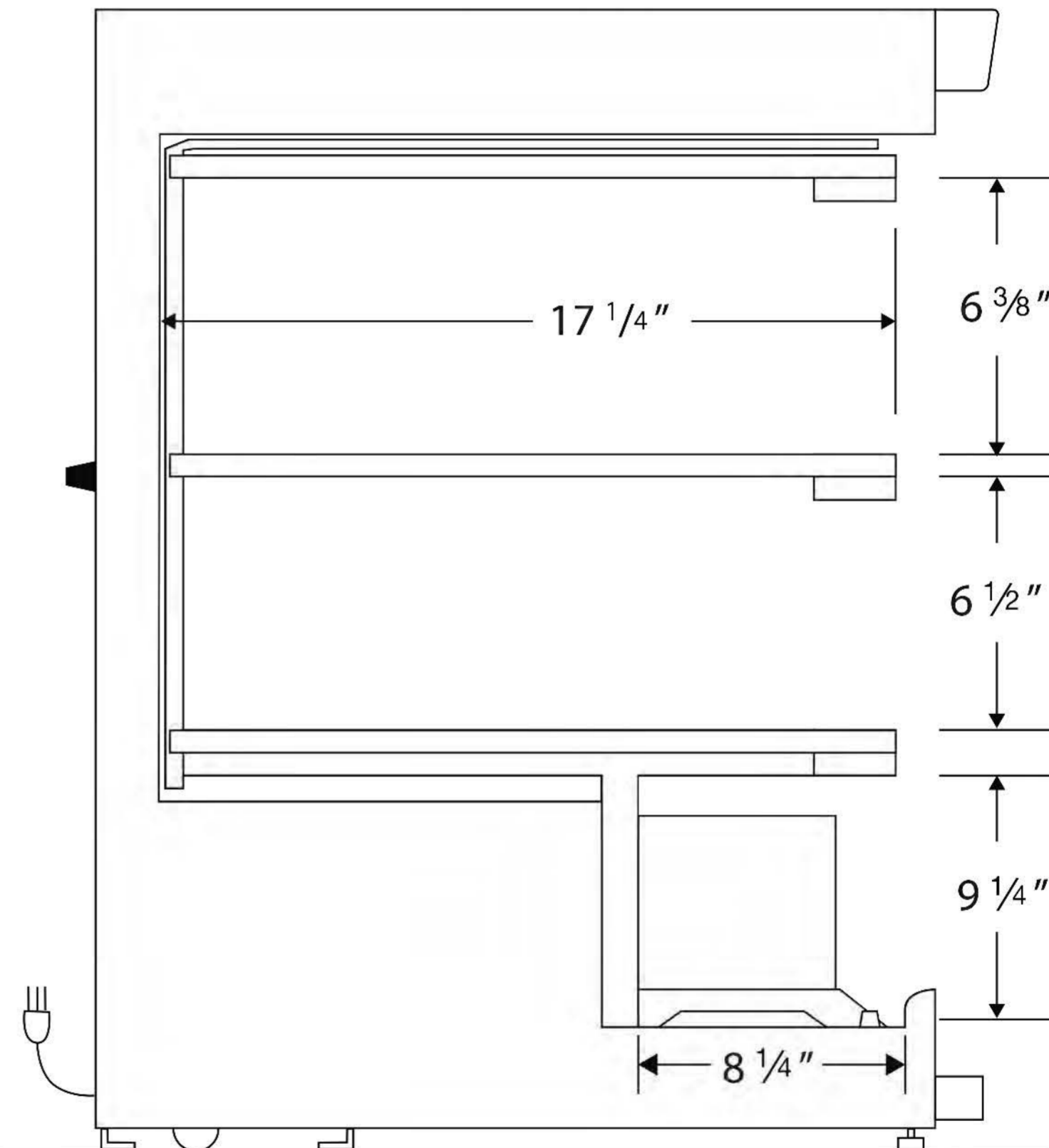
Side View
