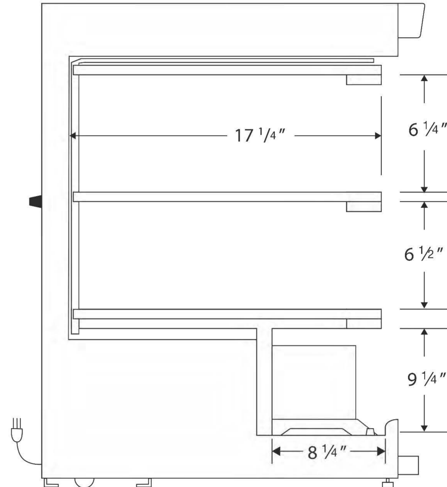
Side View
