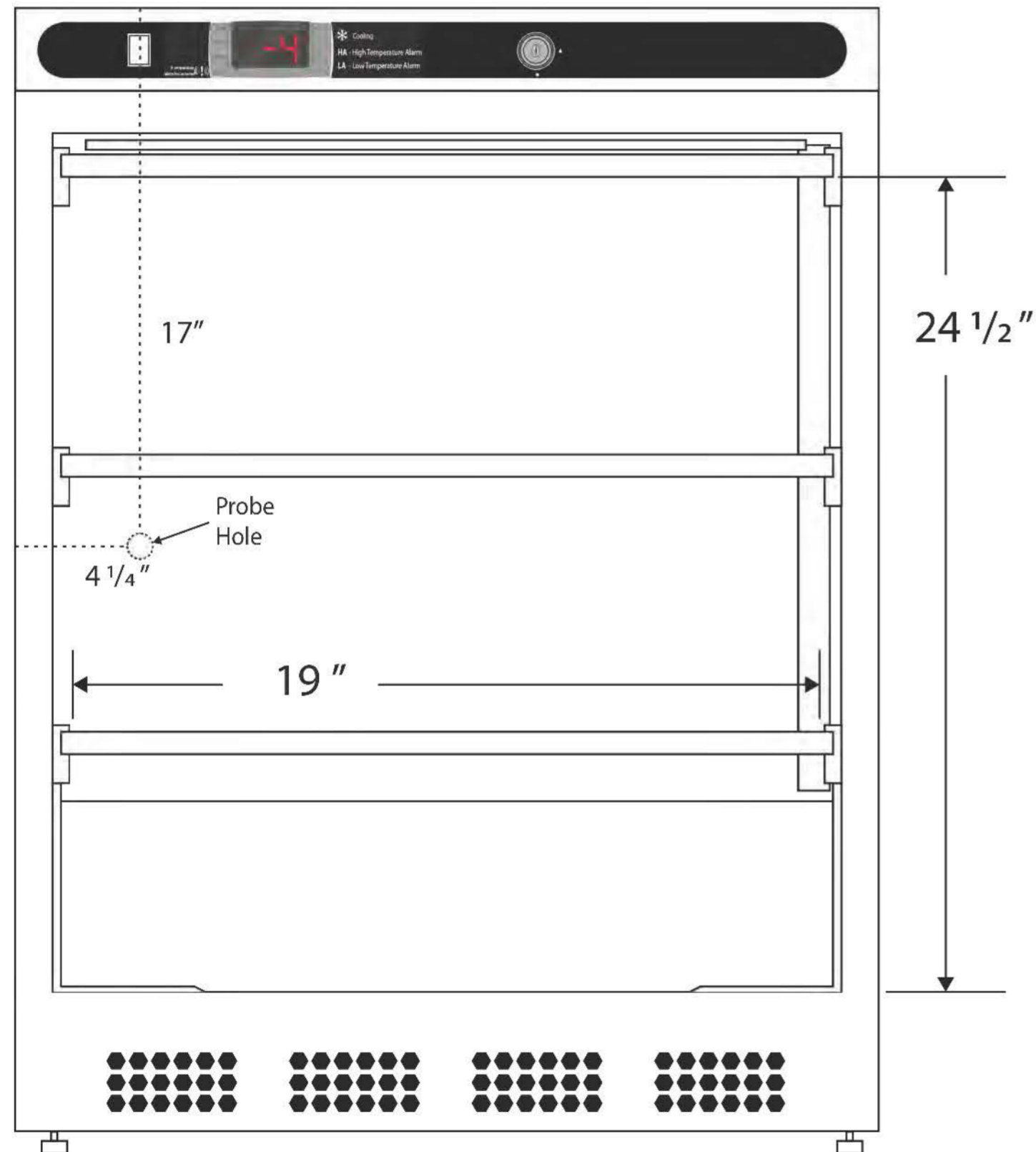
Front View
