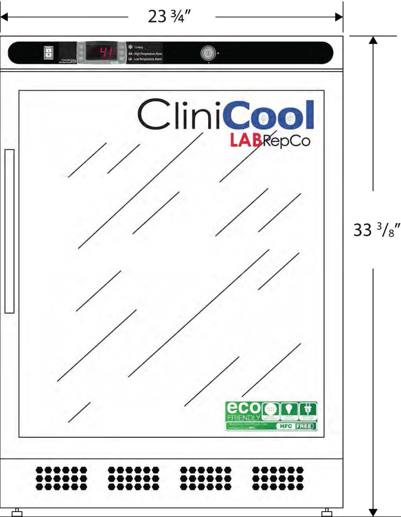
Front View
