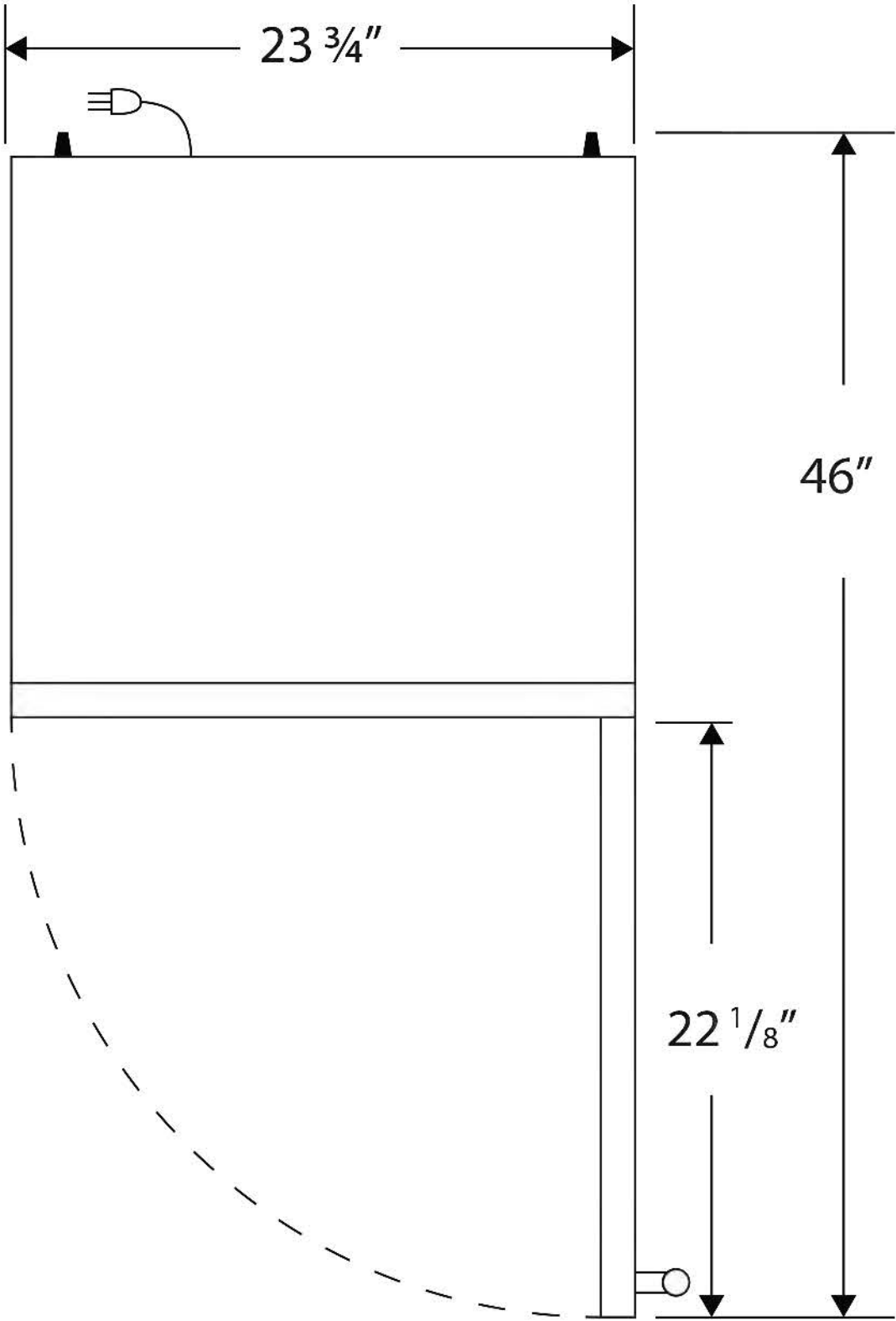
Top View
