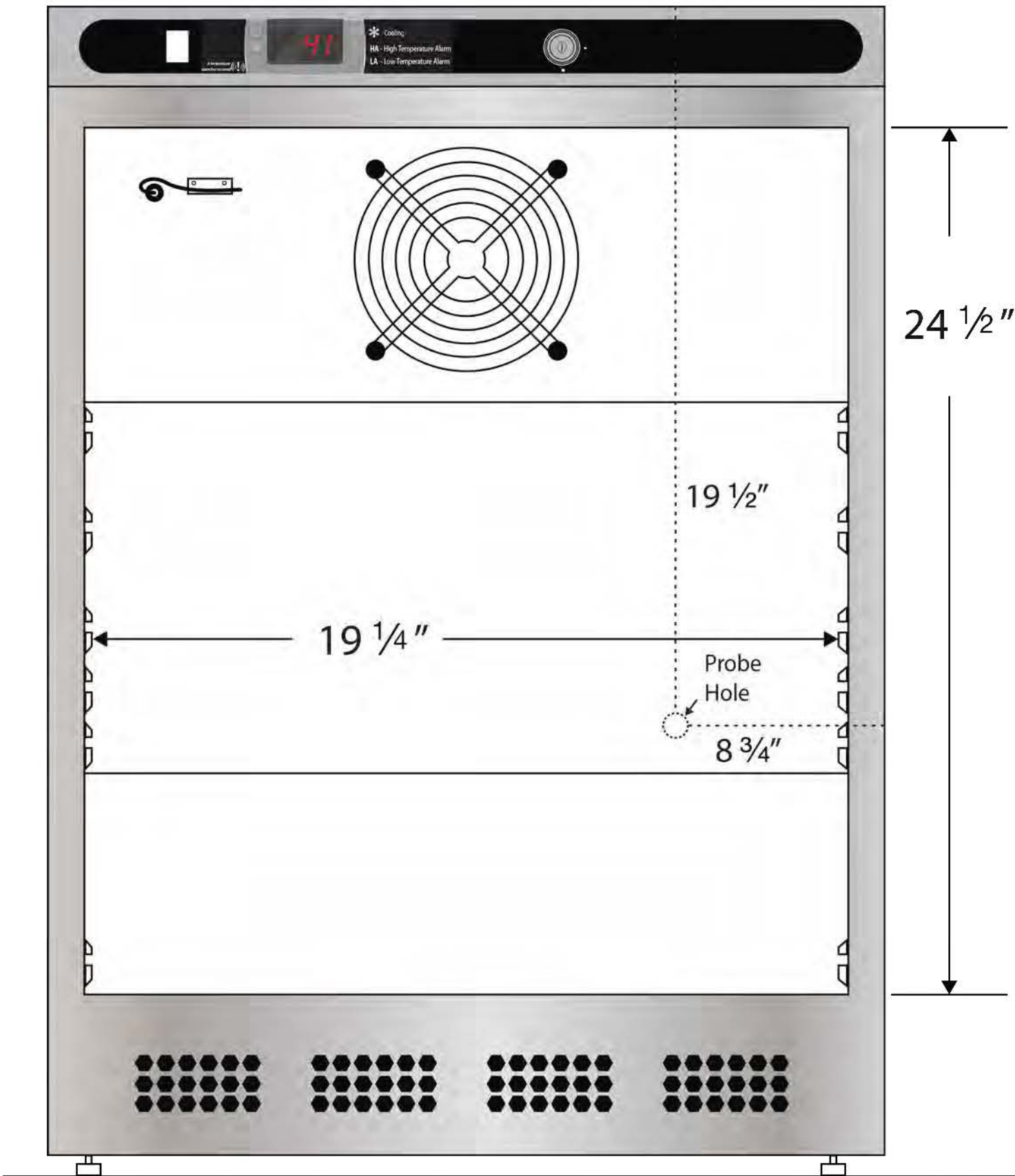
Front View
