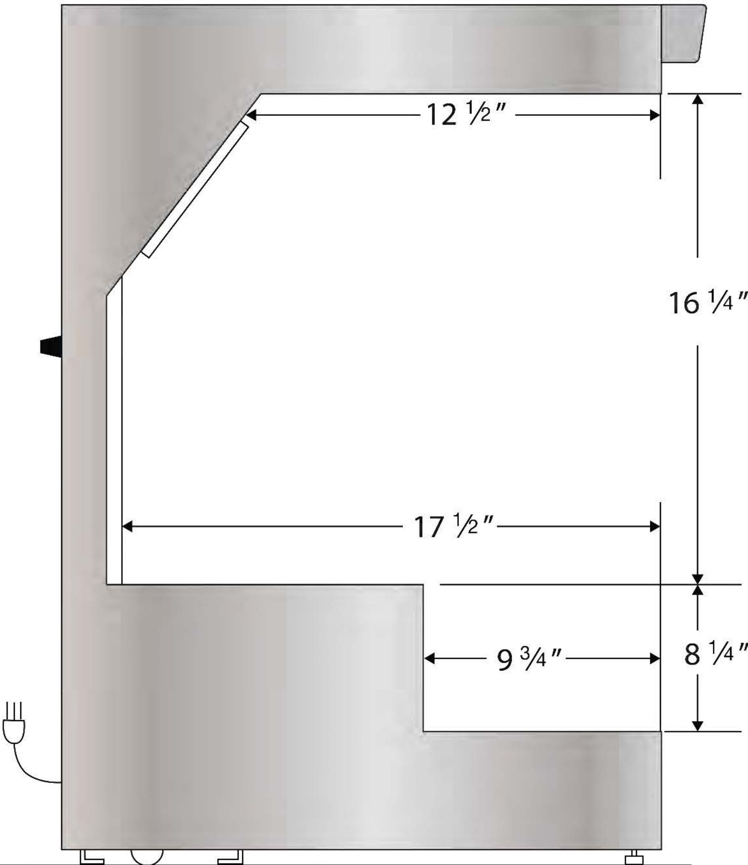
Side View
