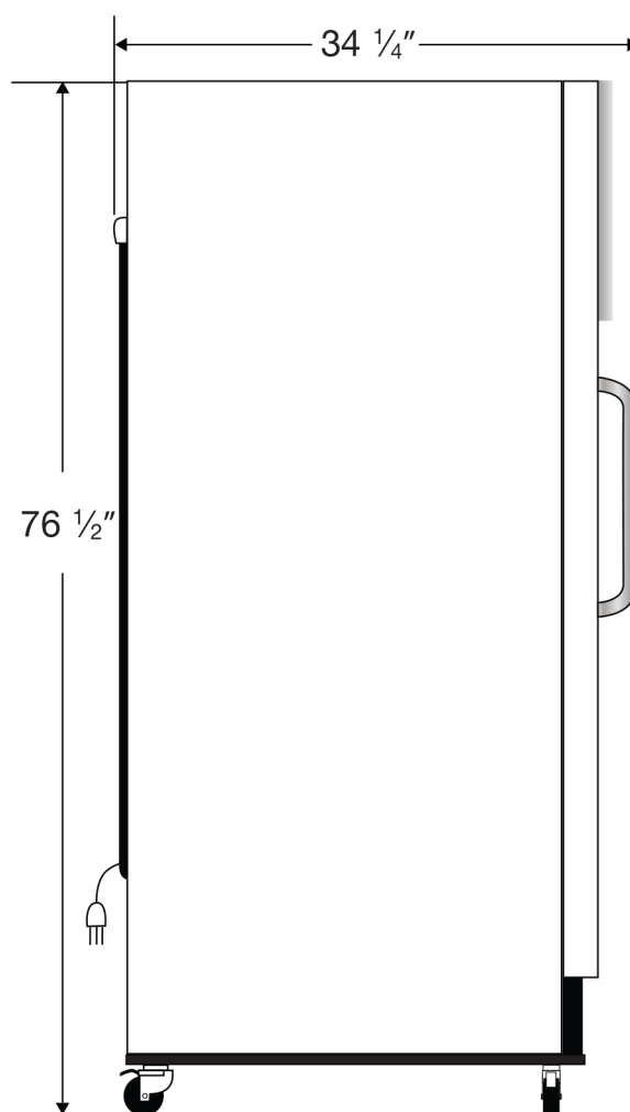
Side View
