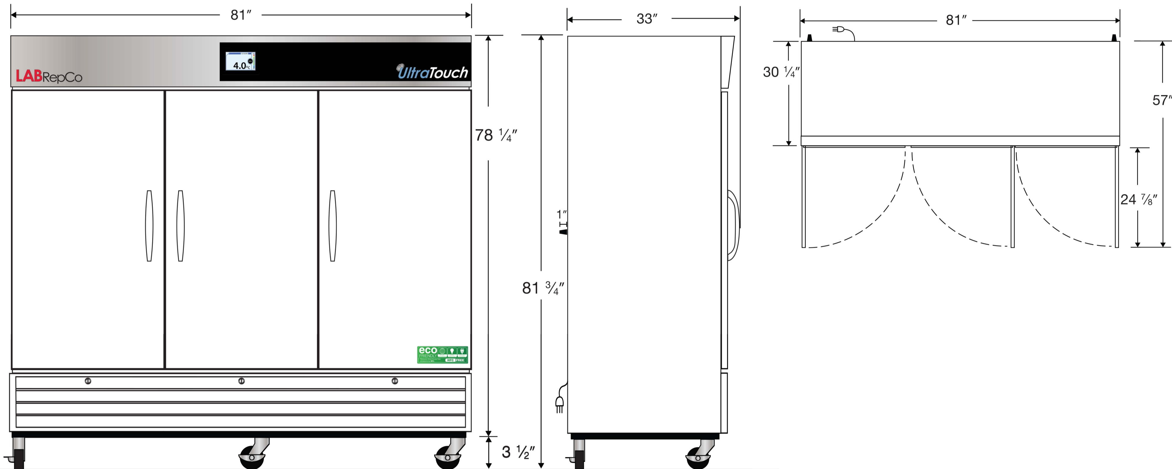
Top View
