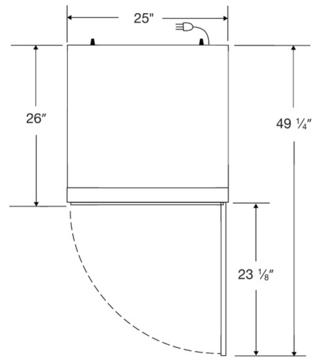
Top View
