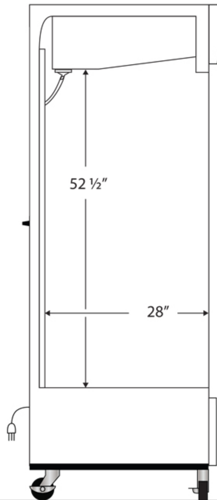
Side View
