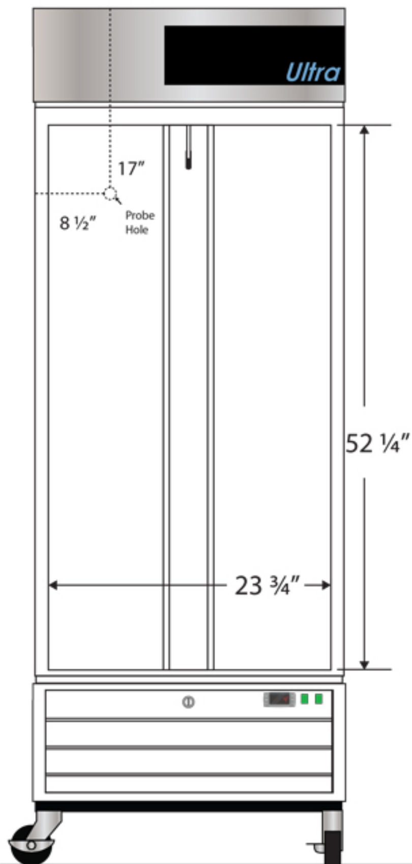
Front View
