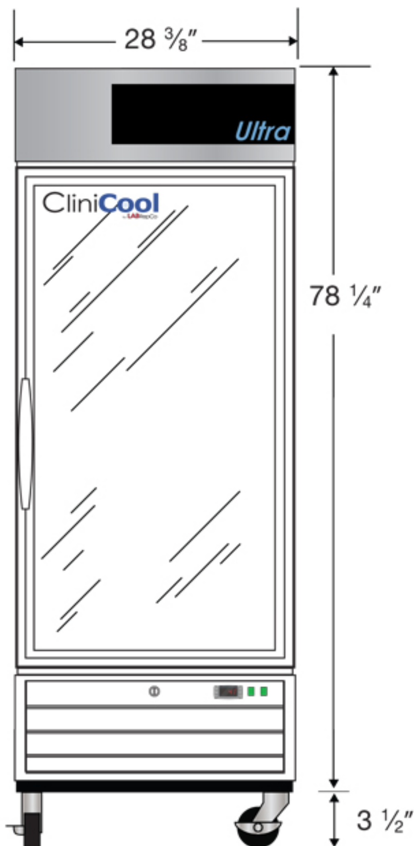
Front View
