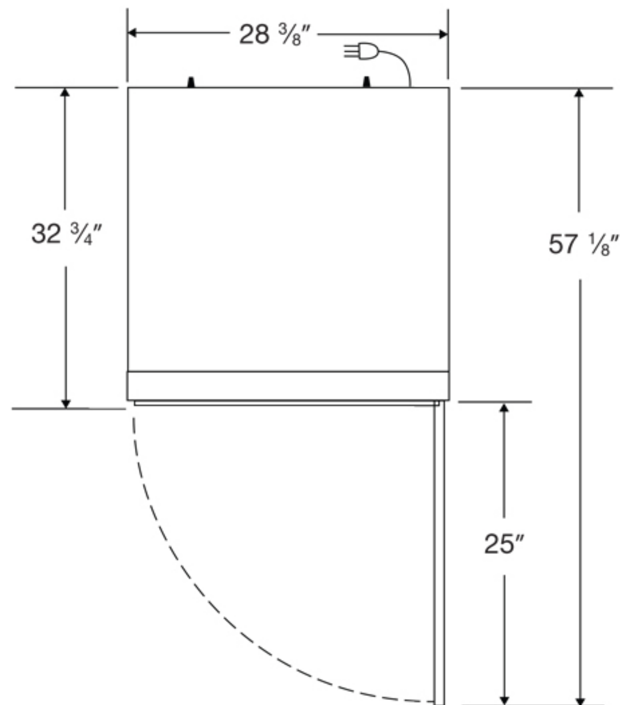
Top View
