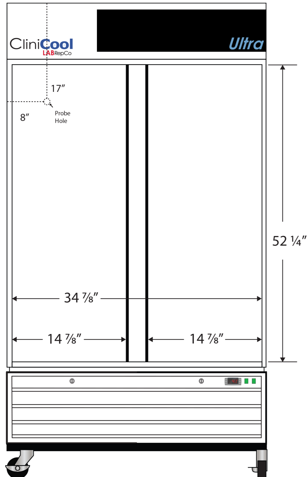
Front View
