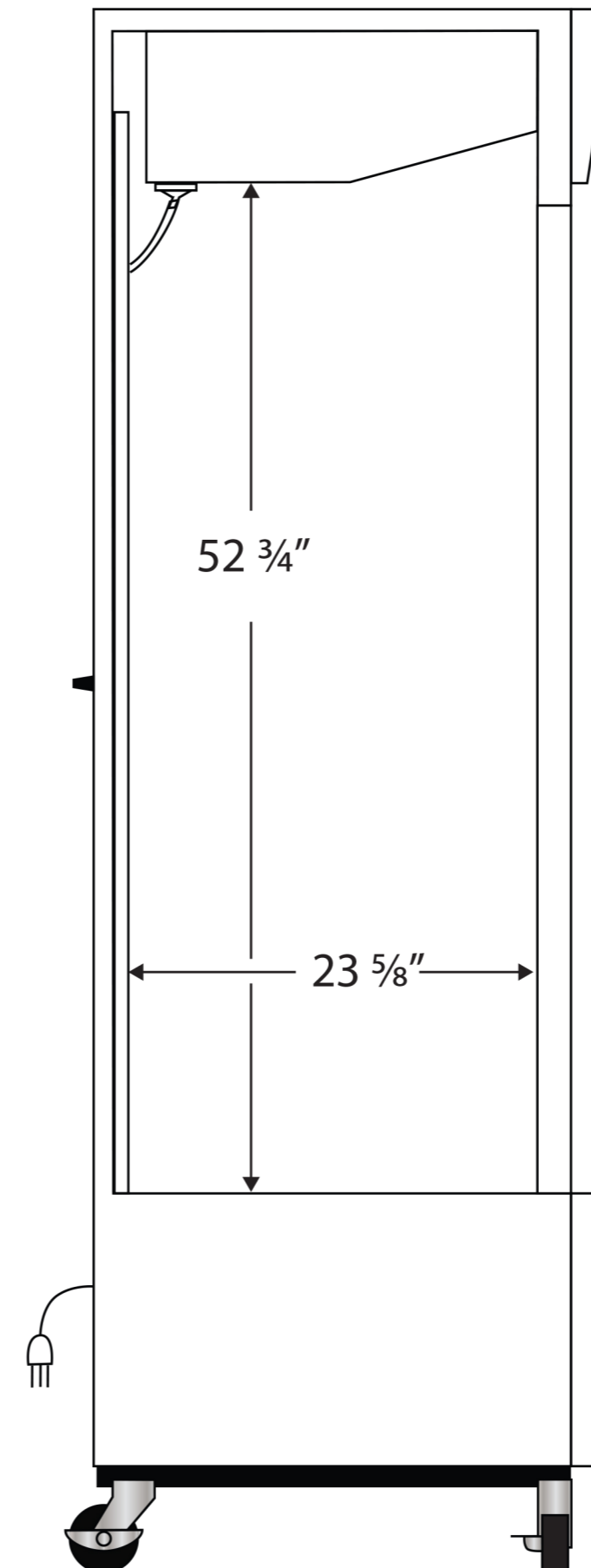
Side View
