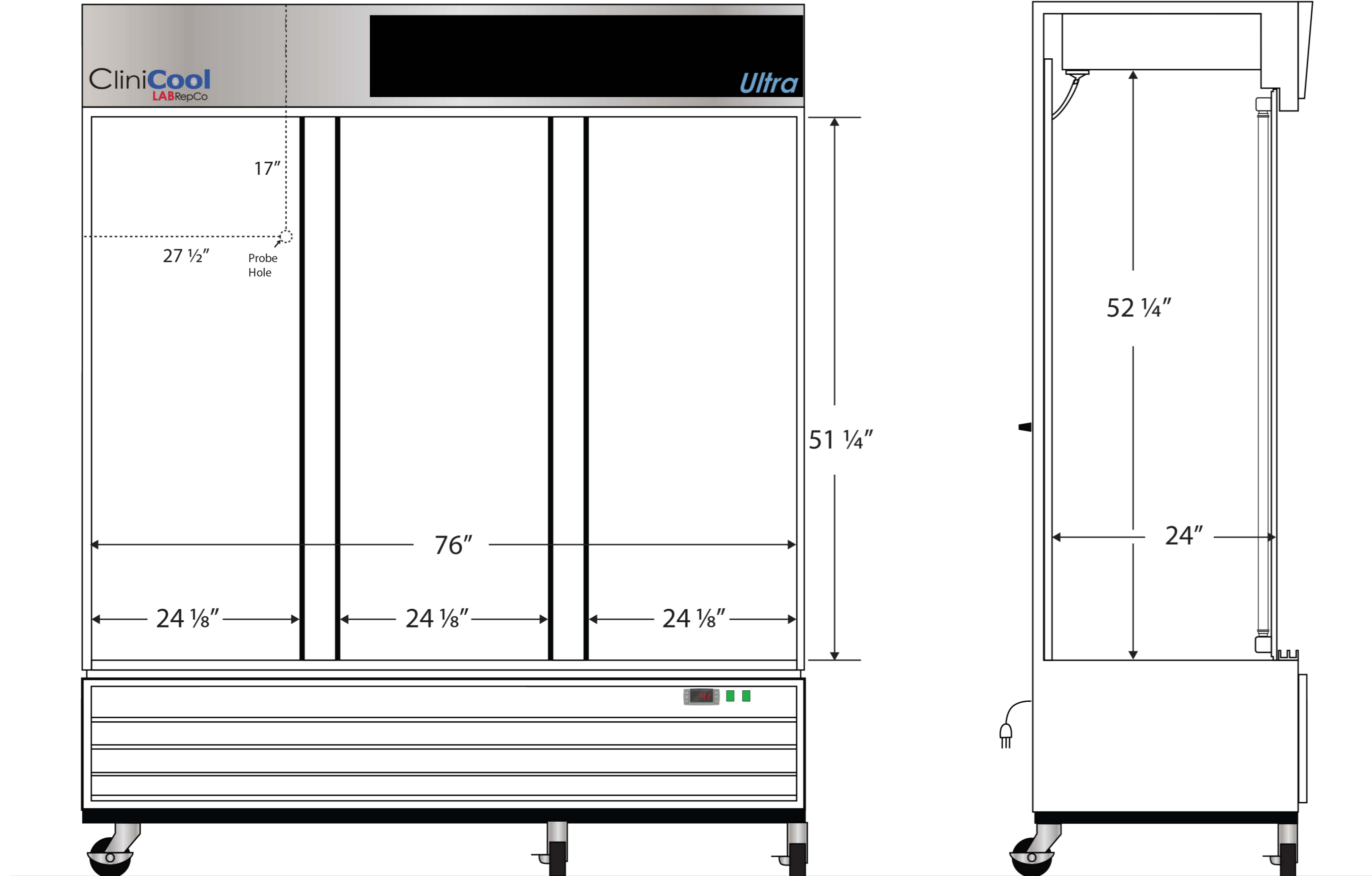
Front View
