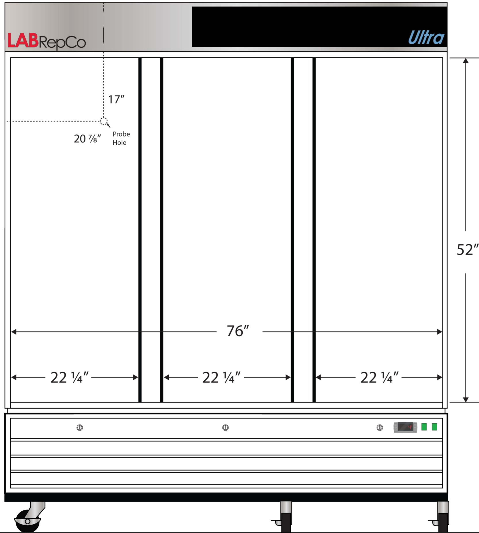
Front View
