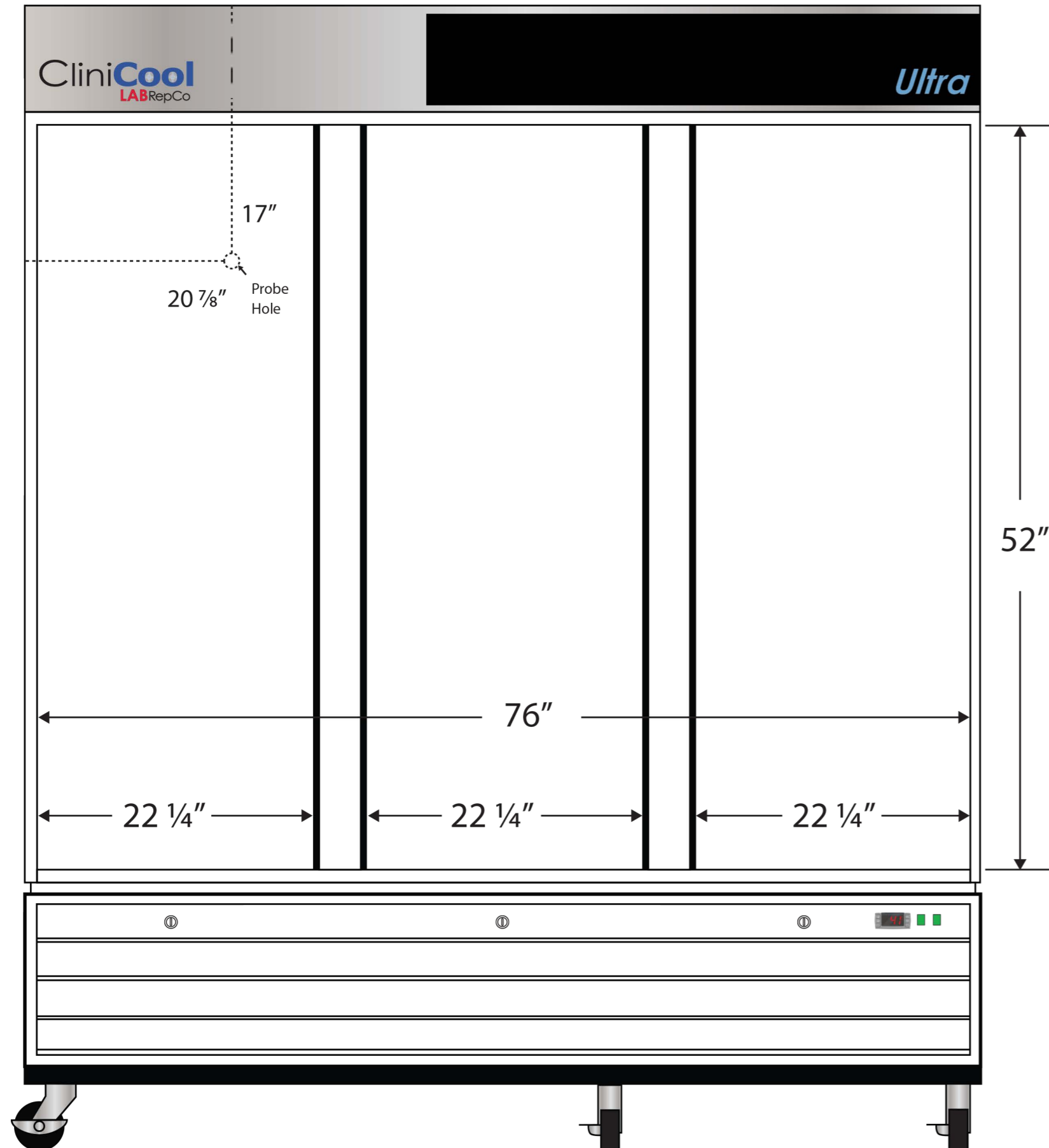
Front View
