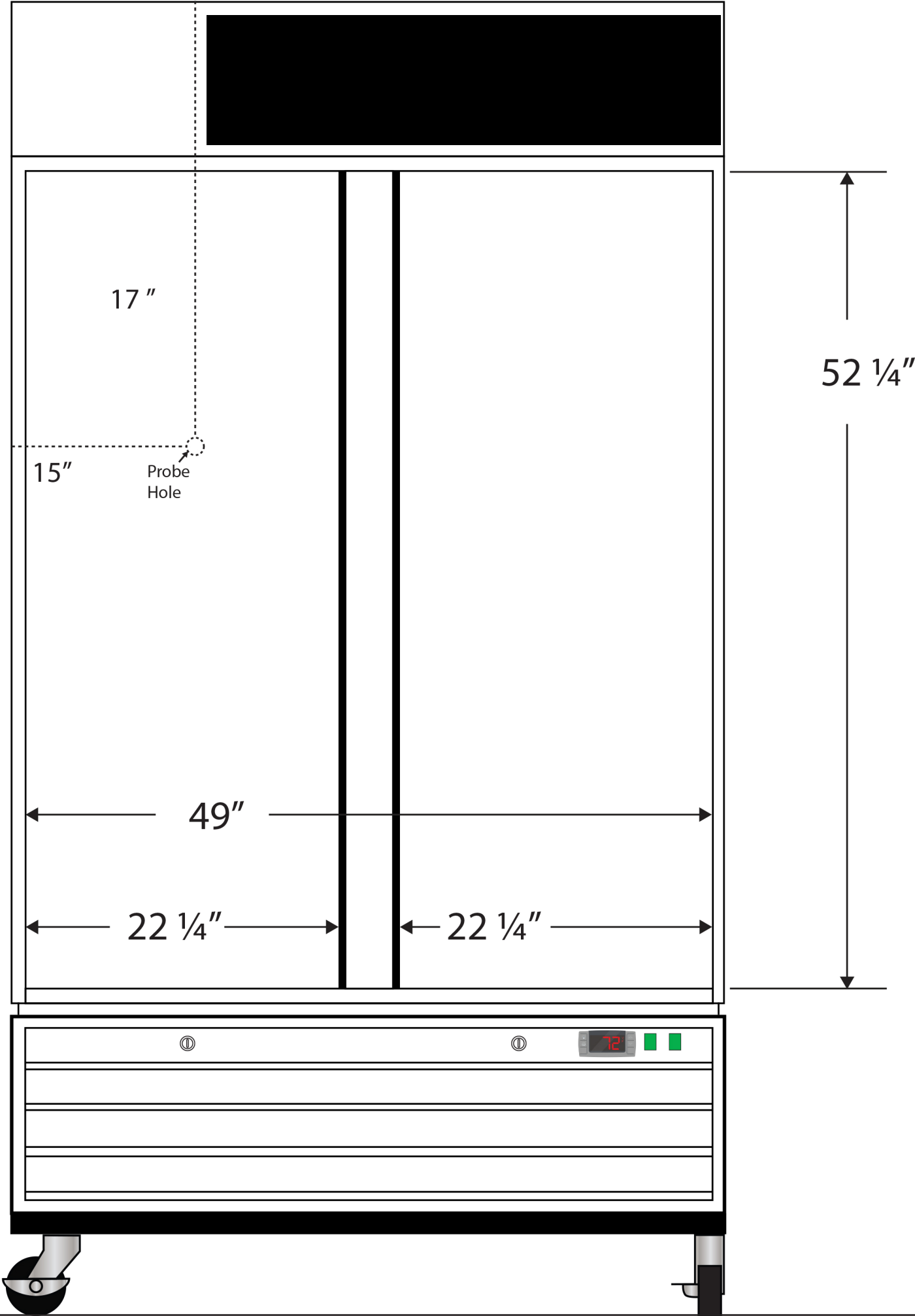
Front View
