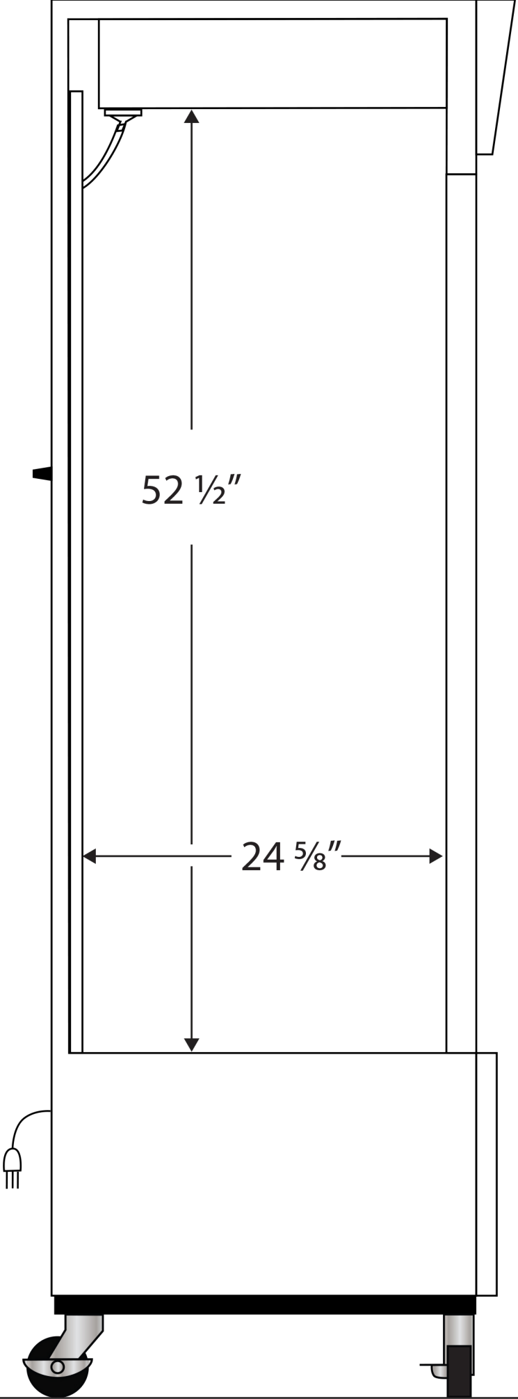
Side View
