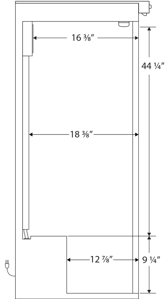
Side View
