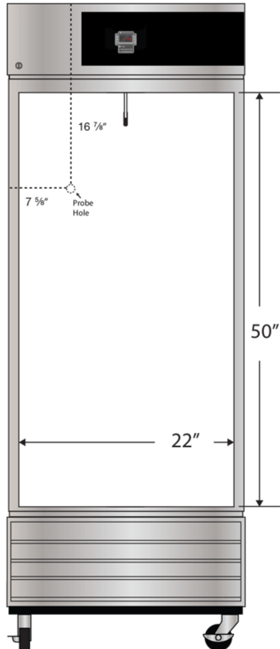
Front View
