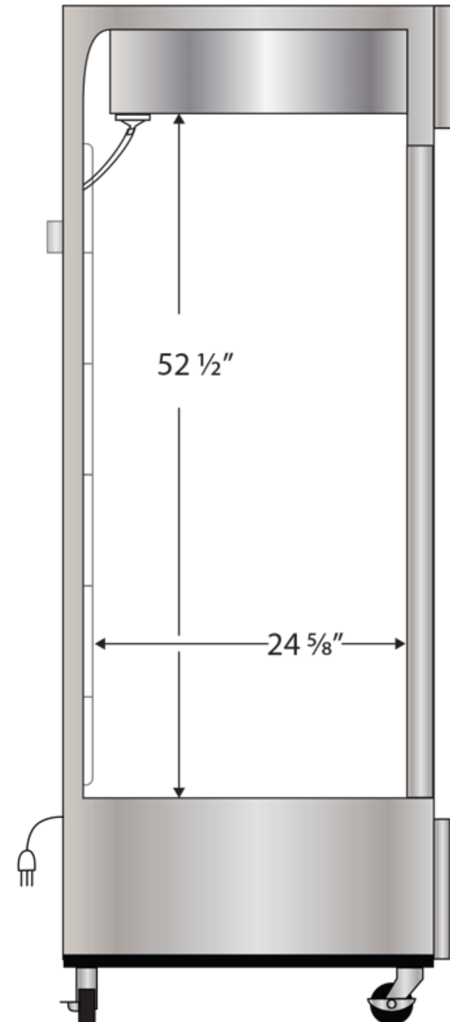
Side View
