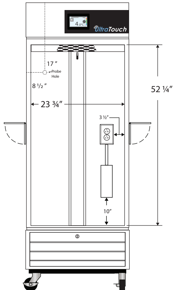
Front View
